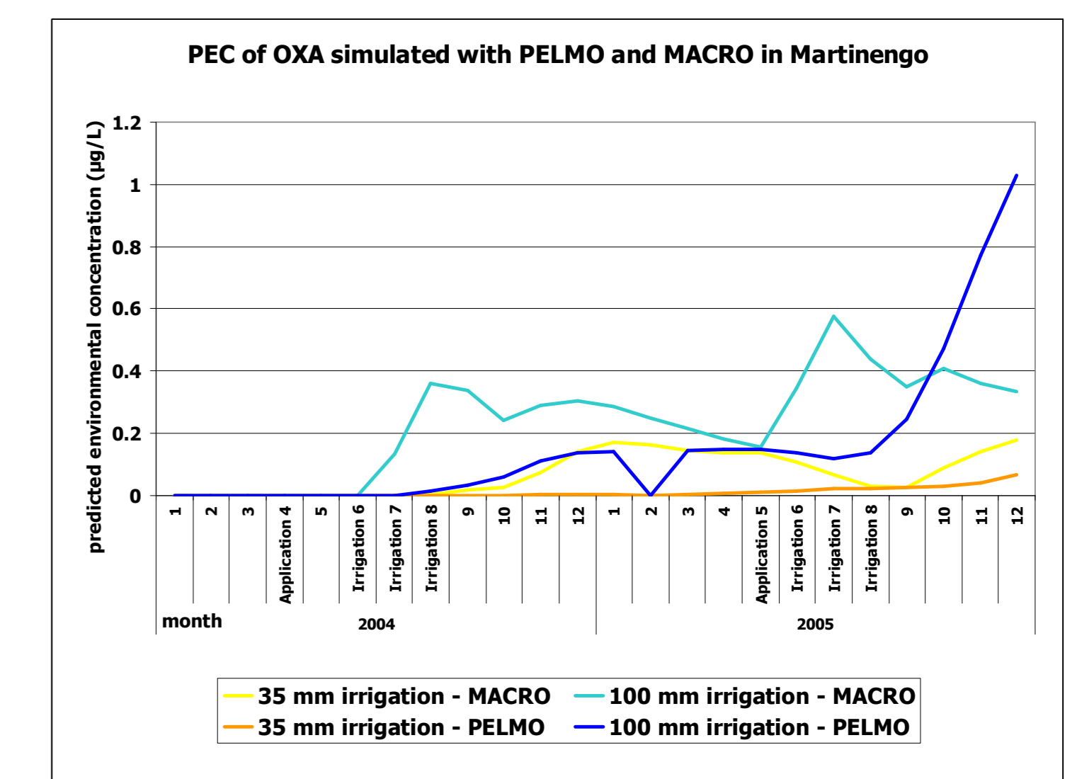
Figure 5: PEC of OXA in leachate below soil core simulated in leachate below soil core with models PELMO and MACRO in different irrigation events (35 and 100 mm).
