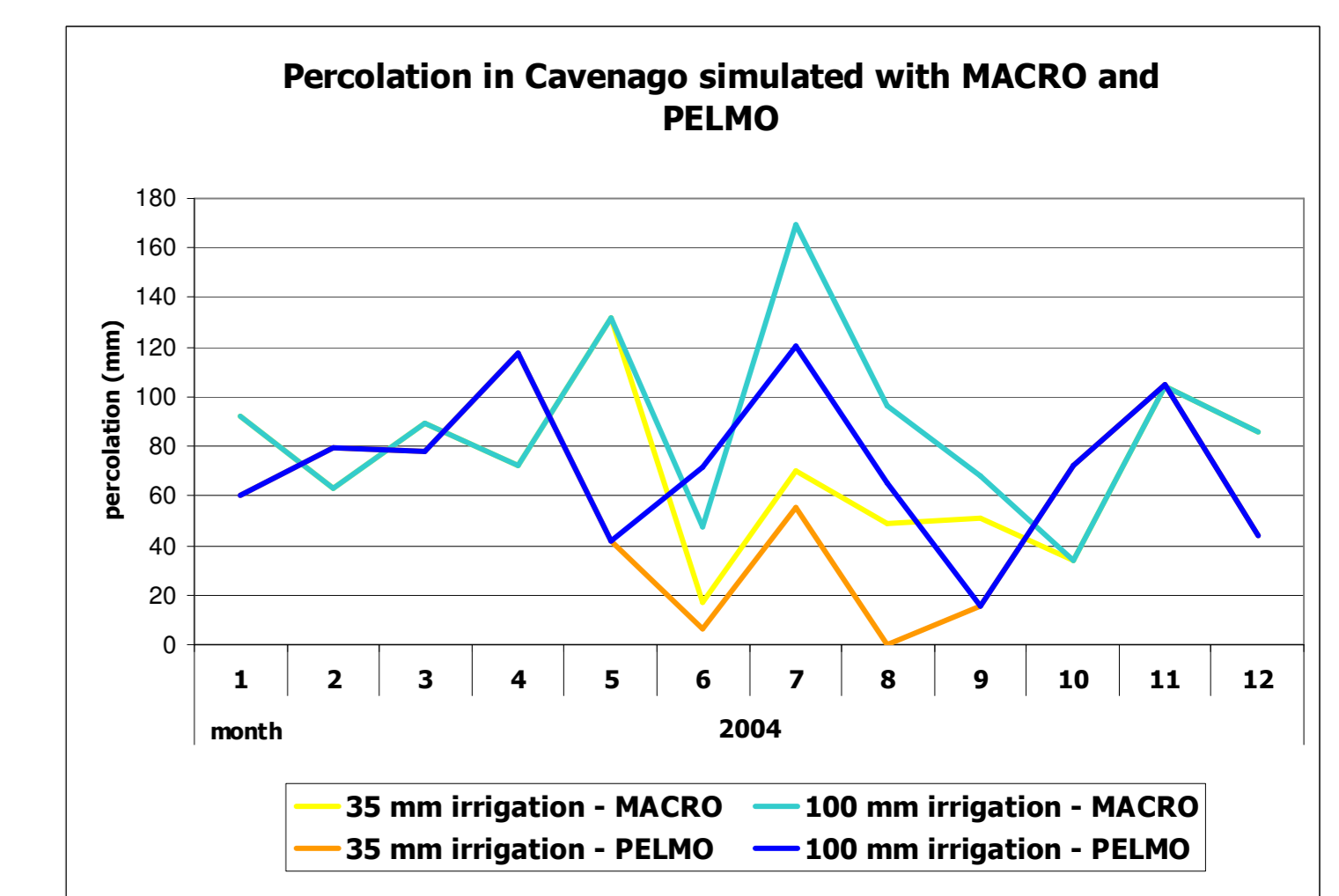
Figure 6: Comparison between simulated percolation with PELMO and MACRO model at amount of 35 and 100 mm irrigation water.
